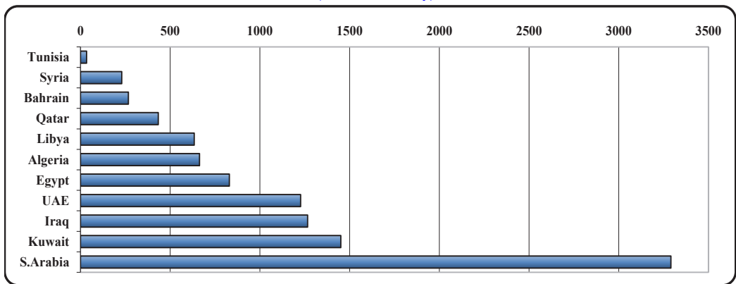
Installed refining capacities in OAPEC Members, 2020-2024 (Thousand b/day)
