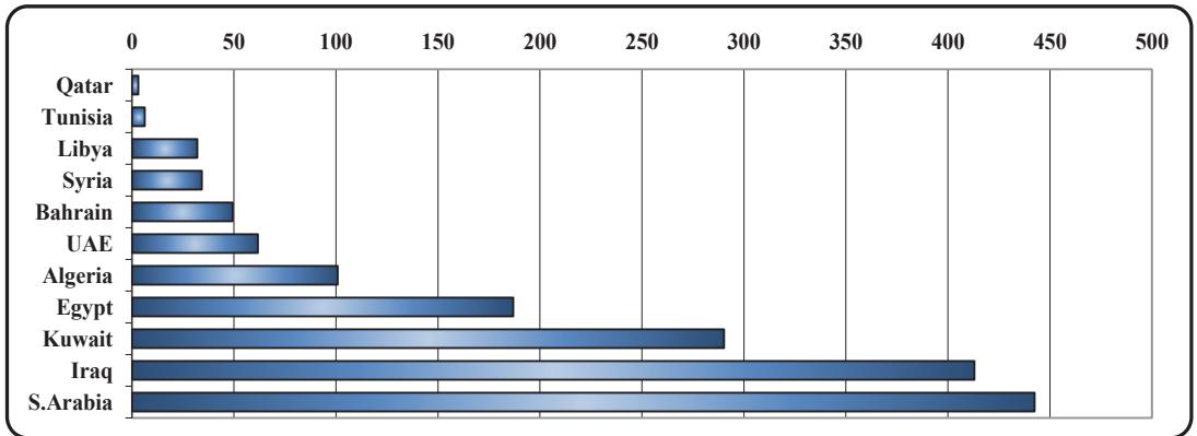
Fuel oil production in OAPEC Members, 2020-2024 (Thousand b/day)
